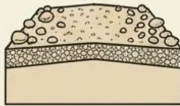
GRAVEL MIGRATES
