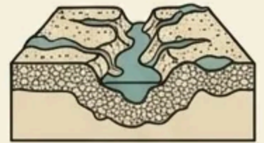
CUT CHANNELS
